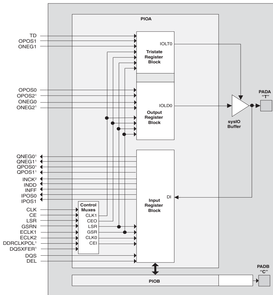
Figure 2-25. PIC Diagram
