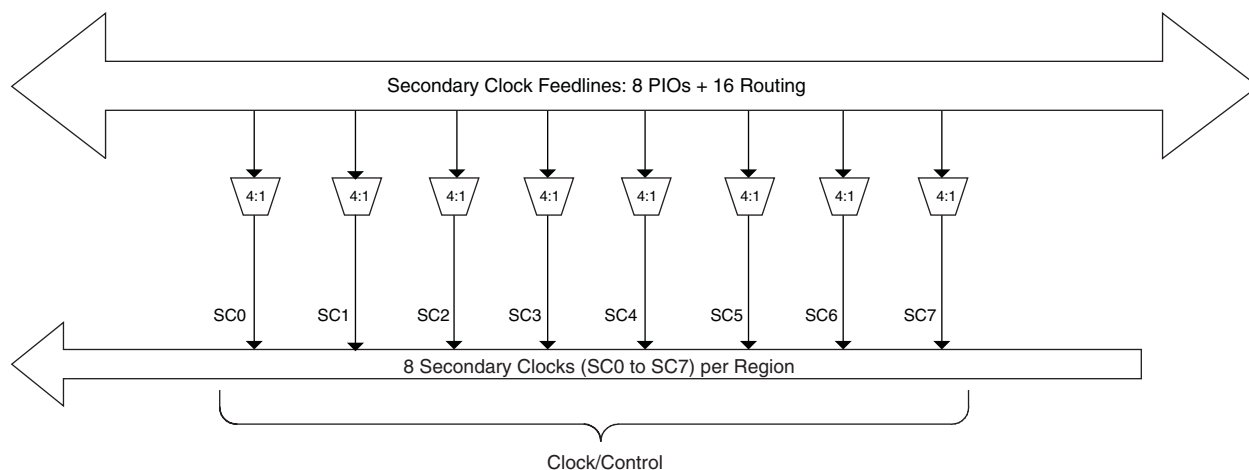
Figure 2-12. Per Region Secondary Clock Selection
