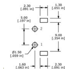
P.C. MOUNTING
