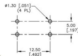
P.C. MOUNTING
