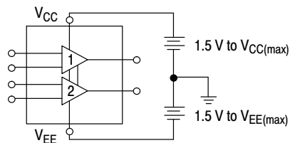
Split Supplies
