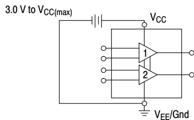
Single Supply
