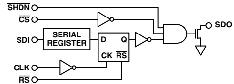
Figure 6. Detail SDO Output Schematic of the AD8403
