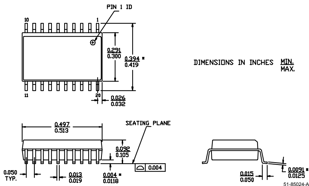
Figure 43: 20-Lead (300-Mil) Molded SOIC S5
