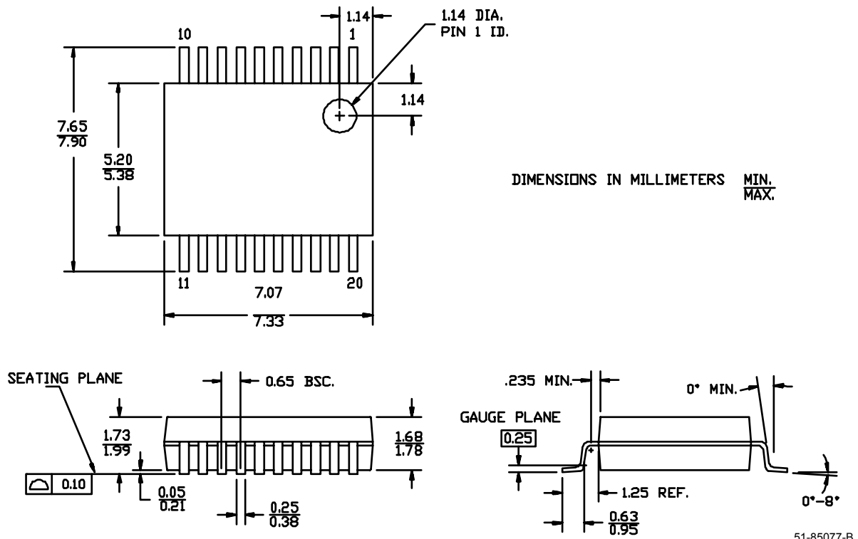
Figure 37: 20-Pin Shrunk Small Outline Package O20
