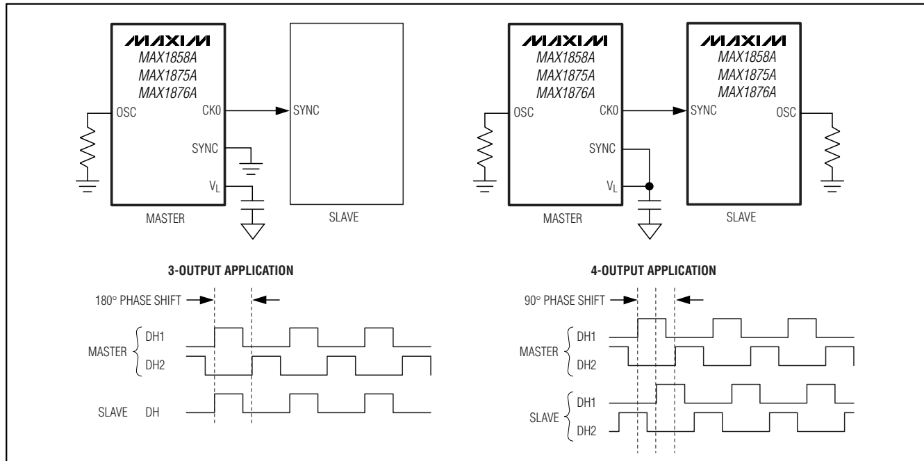
Figure 7. Synchronized Controllers
