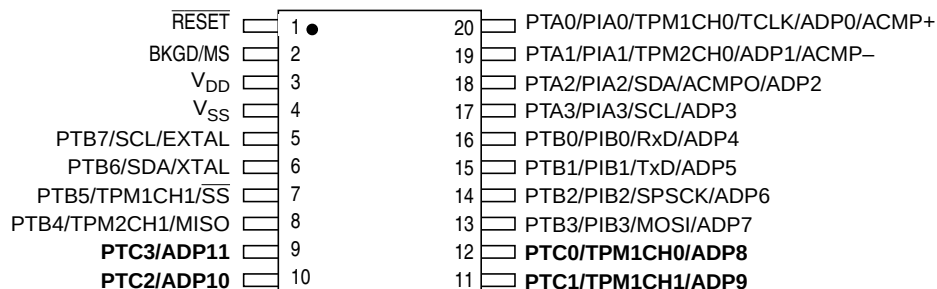
Figure 2-2. 20-Pin TSSOP 1
