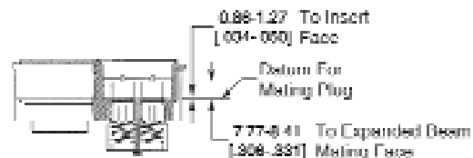
Section Z-Z
