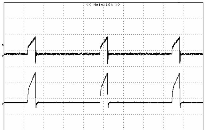
Figure 26: Typical transient response to step load change at 5A/\mu S from 25% to 75% of I_o , max at 12Vin, 5V out (Cout = 1uF ceramic, 10μF tantalum) Top: 100mV/div, 50uS/div, Bottom: 20A/div, 50uS/div
