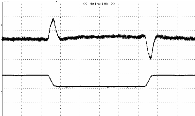
Figure 25: Typical transient response to step load change at 5A/\mu S from 25% to 75% of I_o , max at 12Vin, 3.3V out (Cout = 1uF ceramic, 10μF tantalum) Top: 100mV/div, 50uS/div, Bottom: 20A/div, 50uS/div
