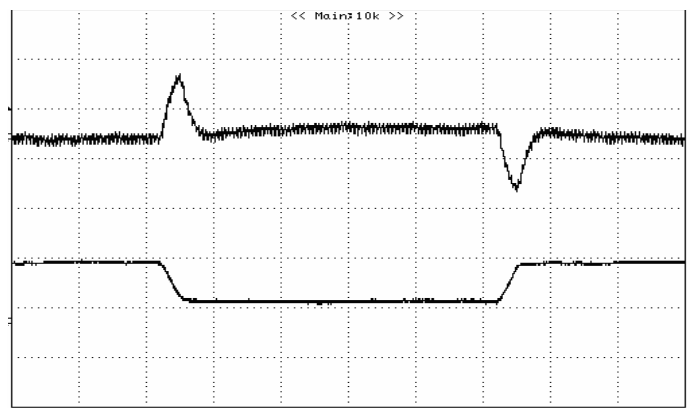
Figure 26: Typical transient response to step load change at 5A/\mu S from 25% to 75% of I_o , max at 12Vin, 5V out (Cout = 1uF ceramic, 10μF tantalum) Top: 100mV/div, 50uS/div, Bottom: 20A/div, 50uS/div
