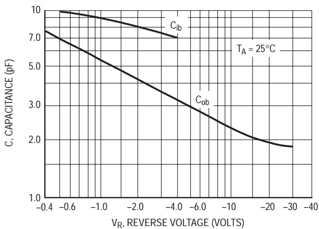
Figure 21. Capacitances
