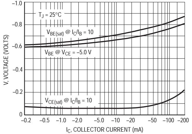
Figure 12. "On" Voltage
