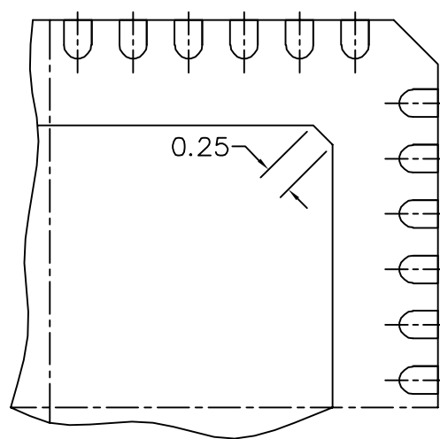
DETAIL M PIN 1 BACKSIDE IDENTIFIER OPTION1
