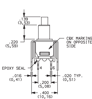
TP11 Models: omit terminal 2.
