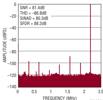
32k Point FFT f_s = 5\text{Mps} , f_{IN} = 2.2\text{MHz}
