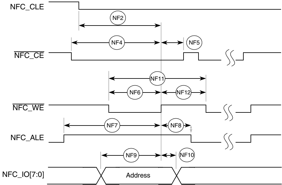
Figure 14. Address latch cycle timing
