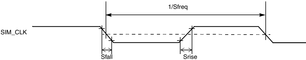
Figure 21. SIM clock timing diagram
