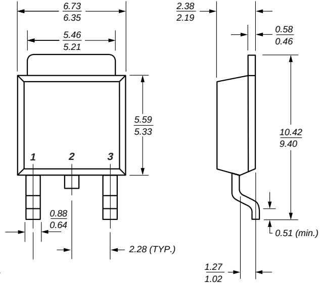
TO-252 (DPAK)
