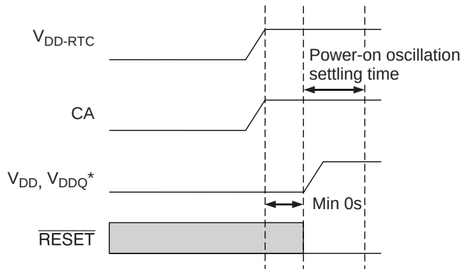
Figure 9.15 Timing When VDD-RTC Power is Off → On
