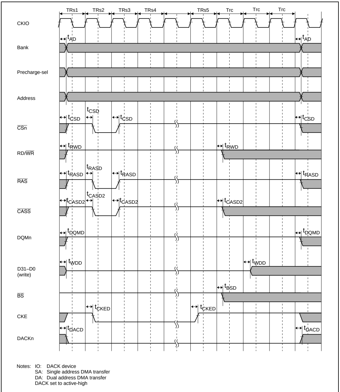
Figure 23.33 Synchronous DRAM Bus Cycle: Self-Refresh (TRC [2:0] = 001)
