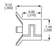
SPEED CLIP 515-0051
