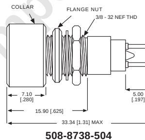
HOLDER WITH COLLAR *
