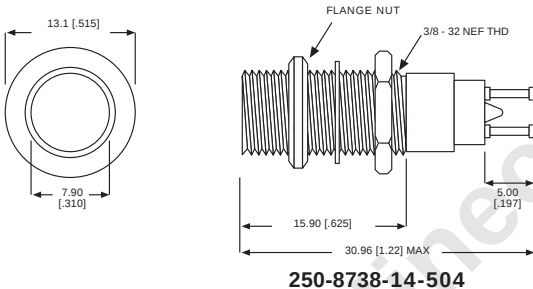
HOLDER WITHOUT COLLAR*
