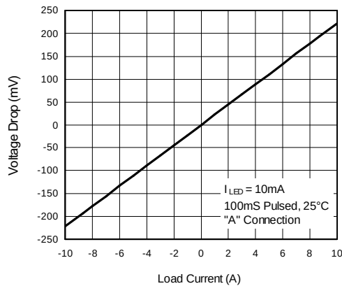
Figure 3. Linearity Characteristics
