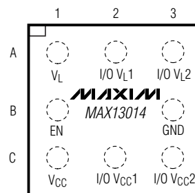
UCSP (BUMPS ON BOTTOM OF DIE)
