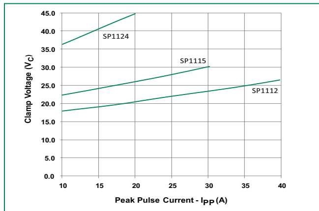
SP1112, SP1115, SP1124 Clamping voltage vs. I_{pp} for 8/20μs waveshape
