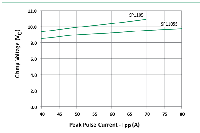
SP1105, SP1105S Clamping voltage vs. I_{pp} for 8/20μs waveshape
