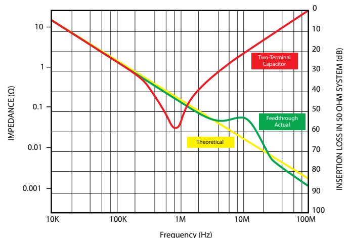
FEEDTHROUGH CAPACITOR PERFORMANCE
