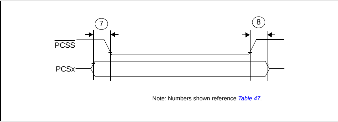
Figure 31. DSPI PCS strobe ( \overline{PCSS} ) timing
