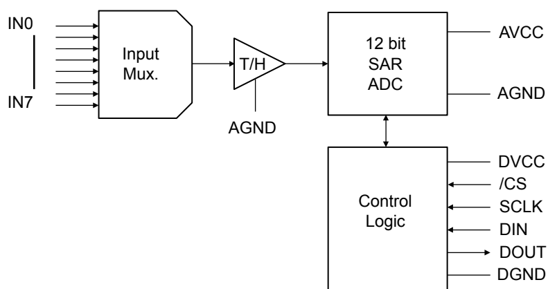
Figure 2. Block diagram
