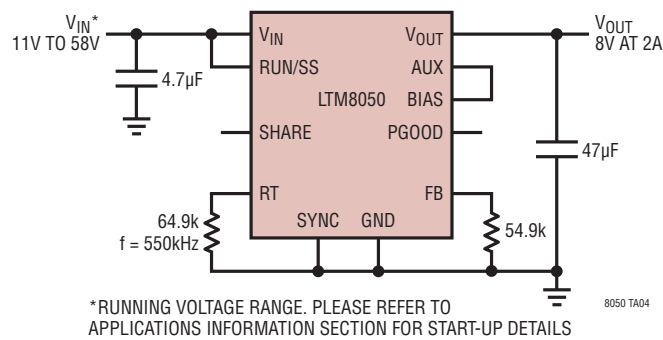
8V Step-Down Converter
