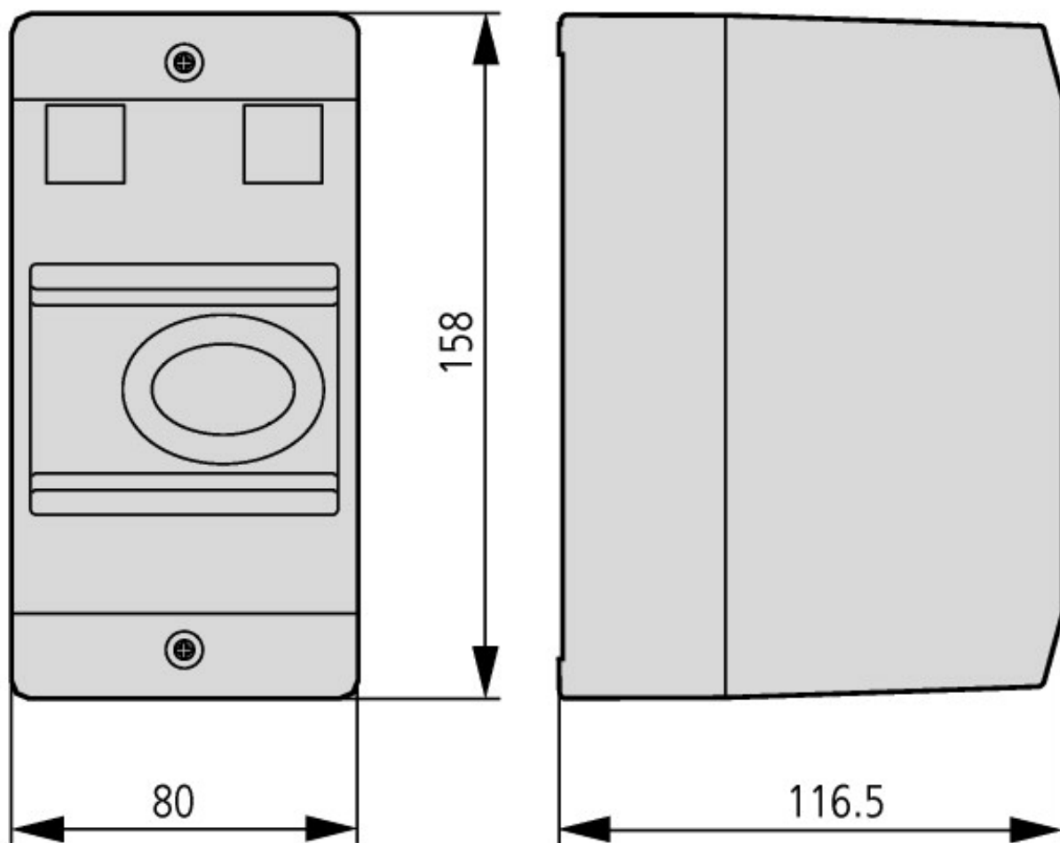
Insulated enclosure for top mounting
