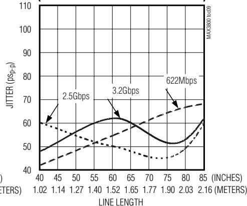
EQUALIZER RESIDUAL JITTER vs. LINE LENGTH (FR-4 6MIL STRIPLINE - SINGLE-ENDED)
