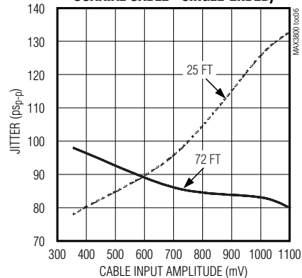
EQUALIZER RESIDUAL JITTER vs. CABLE INPUT AMPLITUDE (RG179B 75Ω COAXIAL CABLE - SINGLE-ENDED)
