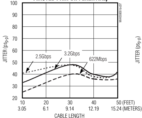
EQUALIZER RESIDUAL JITTER vs. CABLE LENGTH (MADISON #13887 SHIELDED TWISTED PAIR-DIFFERENTIAL)
