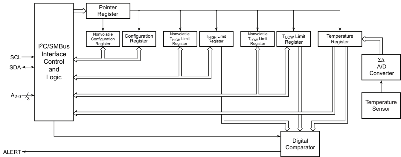
Figure 3-1. Block Diagram
