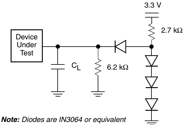
Figure 9. Test Setup
