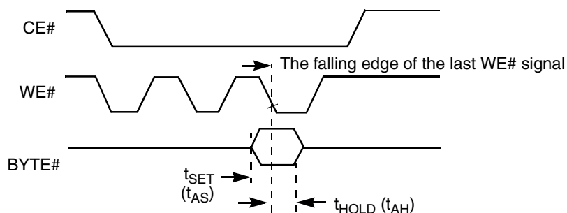
Figure 14. BYTE# Timings for Write Operations
