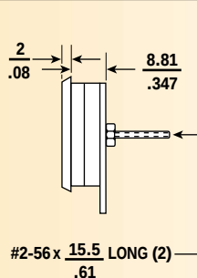
Bezel Mount Side View
