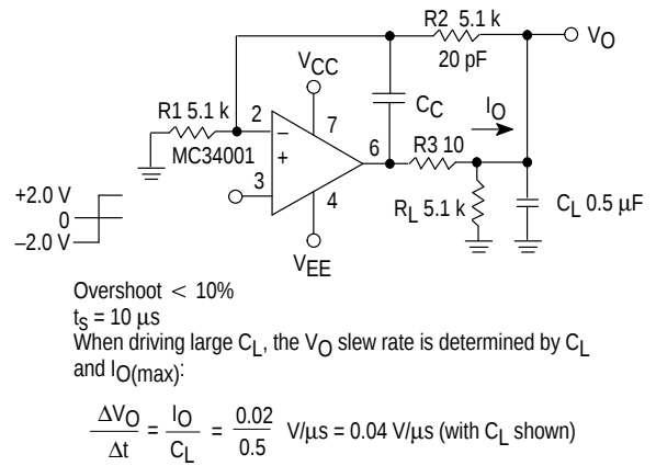
Figure 15. Isolating Large Capacitive Loads
