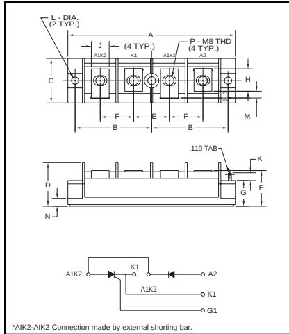
Outline Drawing
