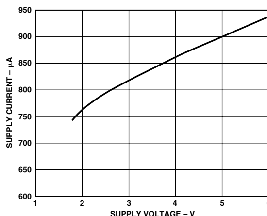
Figure 2. Supply Current per Amplifier vs. Supply Voltage
