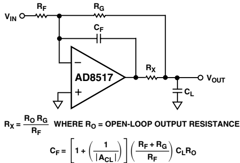
Figure 22. In-the-Loop Compensation Technique for Driving Capacitive Loads
