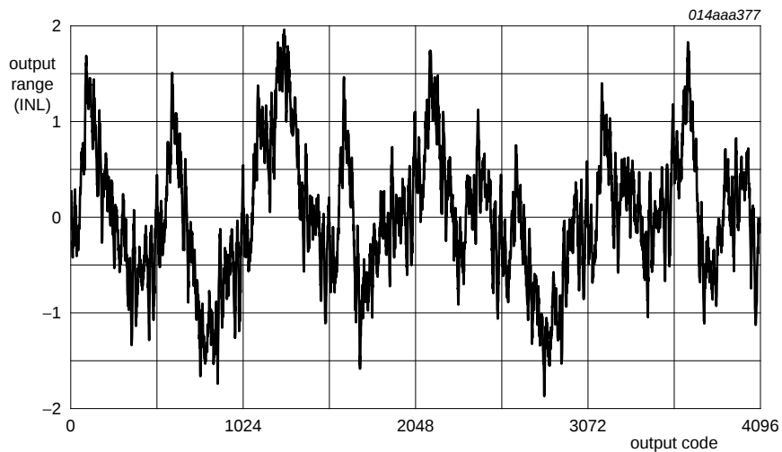
Fig 11. Integral Non-Linearity (INL)
