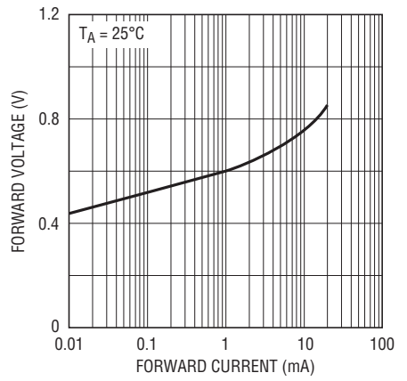
Forward Characteristics
