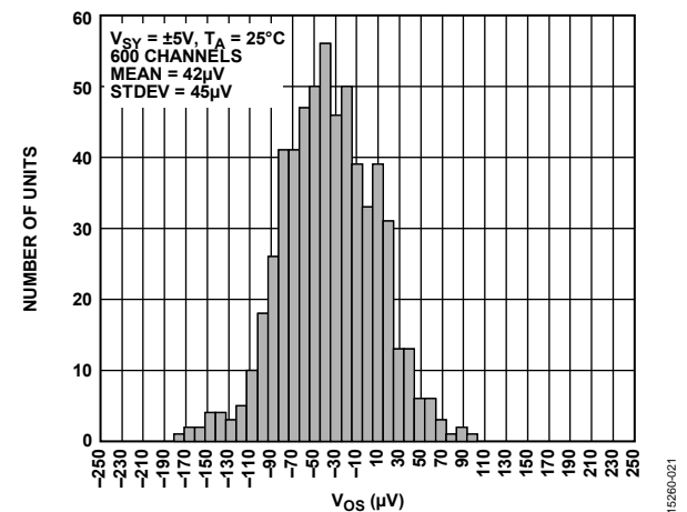
Figure 21. Input Offset Voltage ( V_{OS} ) Distribution, V_{SY} = \pm 5V
