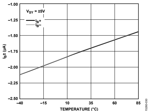
Figure 30. Input Bias Current ( I_{B\pm} ) vs. Temperature, V_{SY} = \pm 5V
