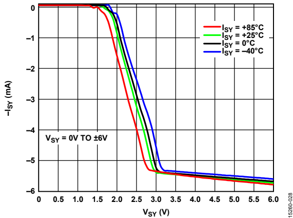
Figure 28. Supply Current ( -I_{SY} ) vs. Supply Voltage ( V_{SY} )
