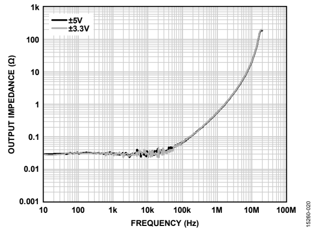
Figure 20. Enabled Output Impedance vs. Frequency
