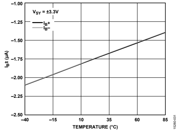
Figure 31. Input Bias Current ( I_{B\pm} ) vs. Temperature, V_{SY} = \pm 3.3V
