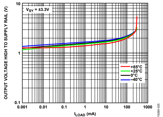
Figure 25. Output Voltage High ( V_{OH} ) to Supply Rail vs. Load Current ( I_{LOAD} ), V_{SY} = \pm 3.3\text{ V}
