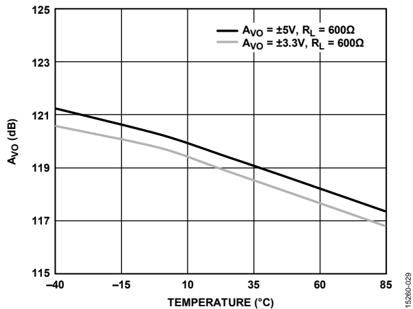
Figure 29. Open-Loop Gain ( A_{VO} ) vs. Temperature
