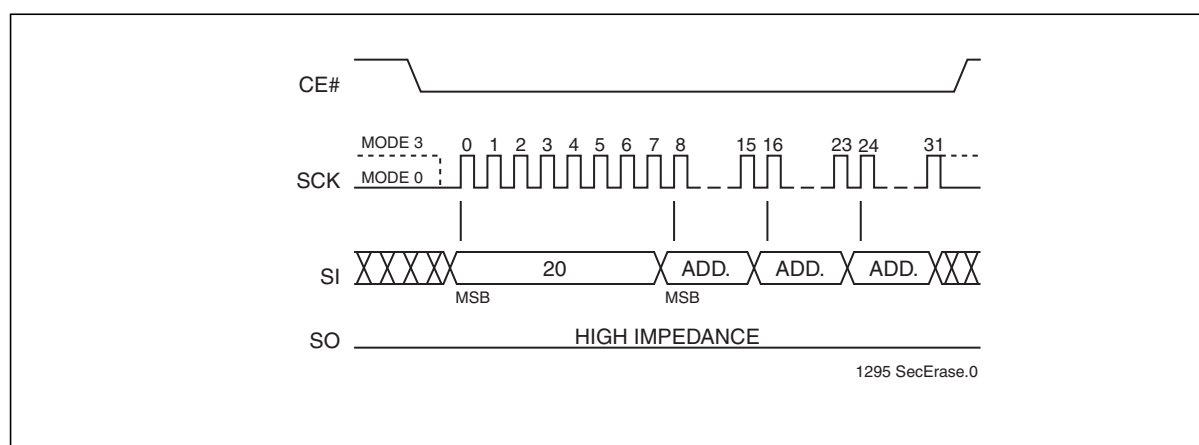
Figure 12: Sector-Erase Sequence
