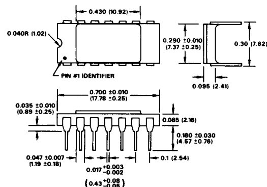
TO-116 "D" PIN CONFIGURATIONS TOP VIEW
