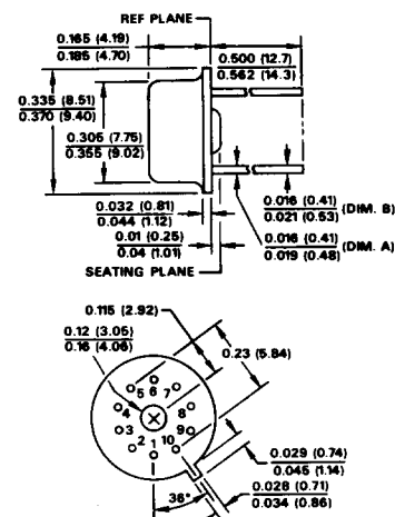
TO-100 "H"
