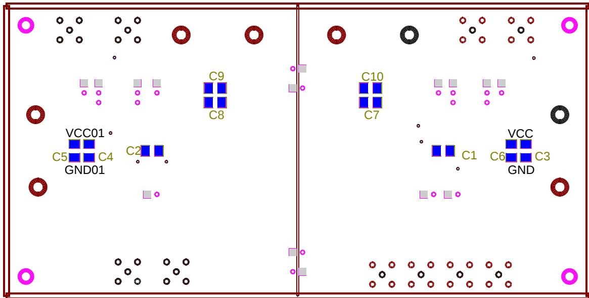
Figure 3–5. Bottom Layer
