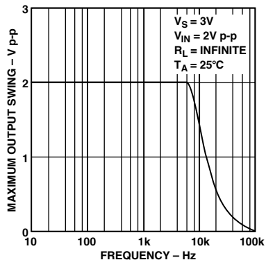
TPC 20. Maximum Output Swing vs. Frequency
