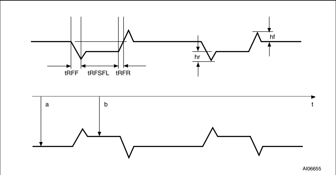
Figure 4. 10% modulation waveform
