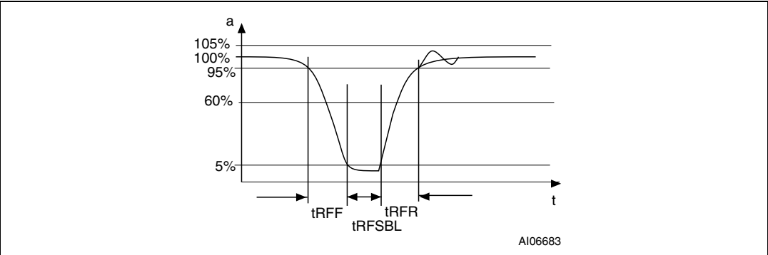
Figure 3. 100% modulation waveform
