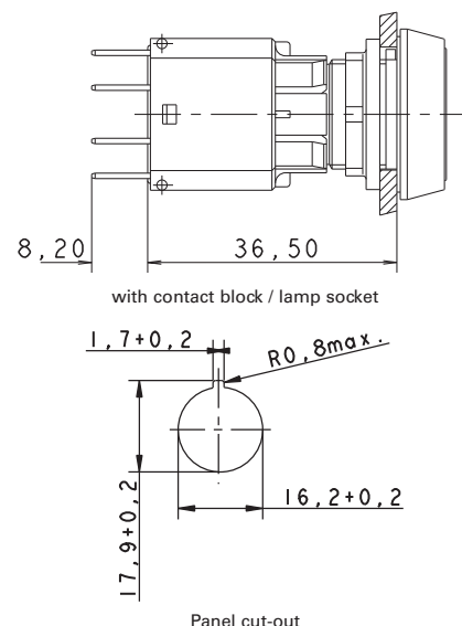
Panel cut-out
