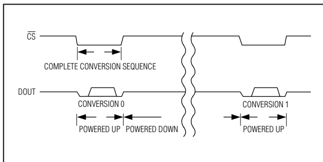
Figure 9. Shutdown Sequence
