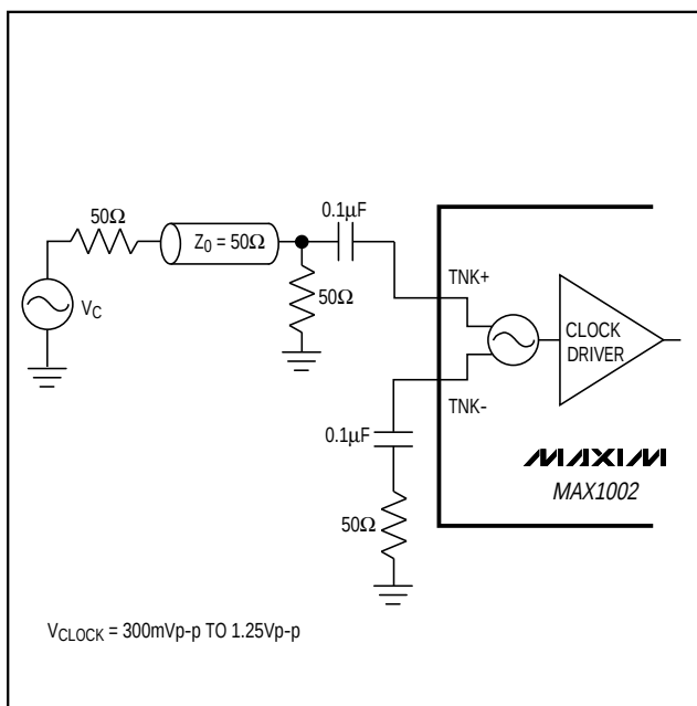
Figure 7. External-Clock-Drive Circuit
