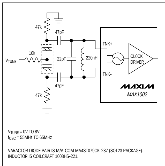
Figure 6. Tank-Resonator Oscillator
