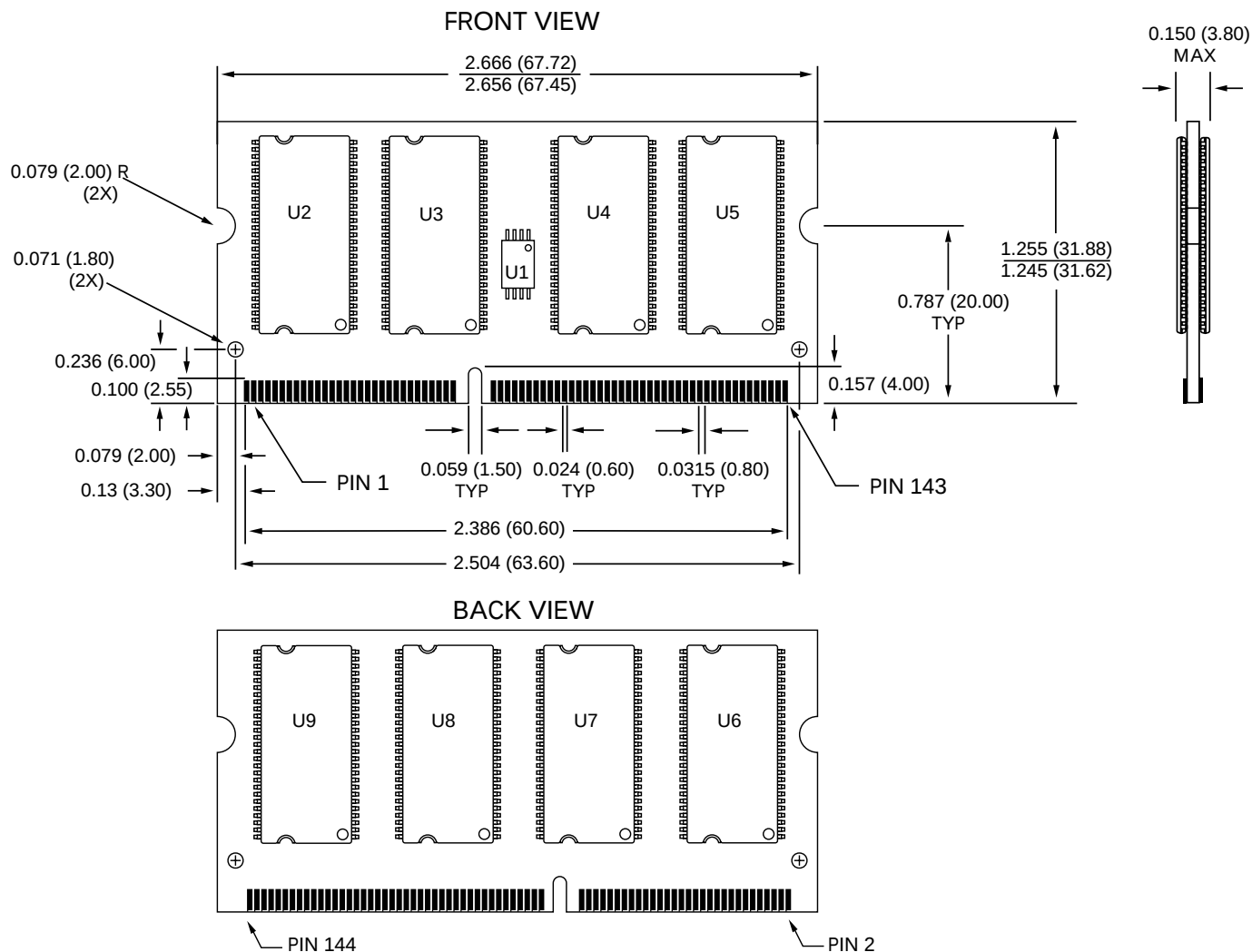
Figure 10: 144-Pin SODIMM
