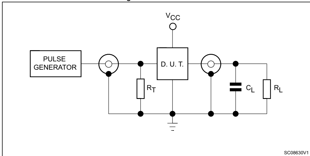
Figure 9. Test circuit
