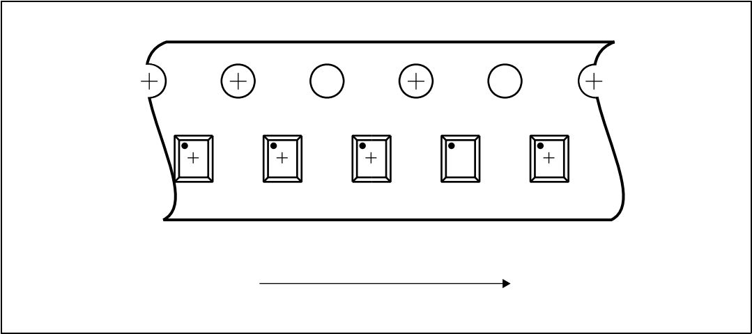
Figure 16. Tape orientation
