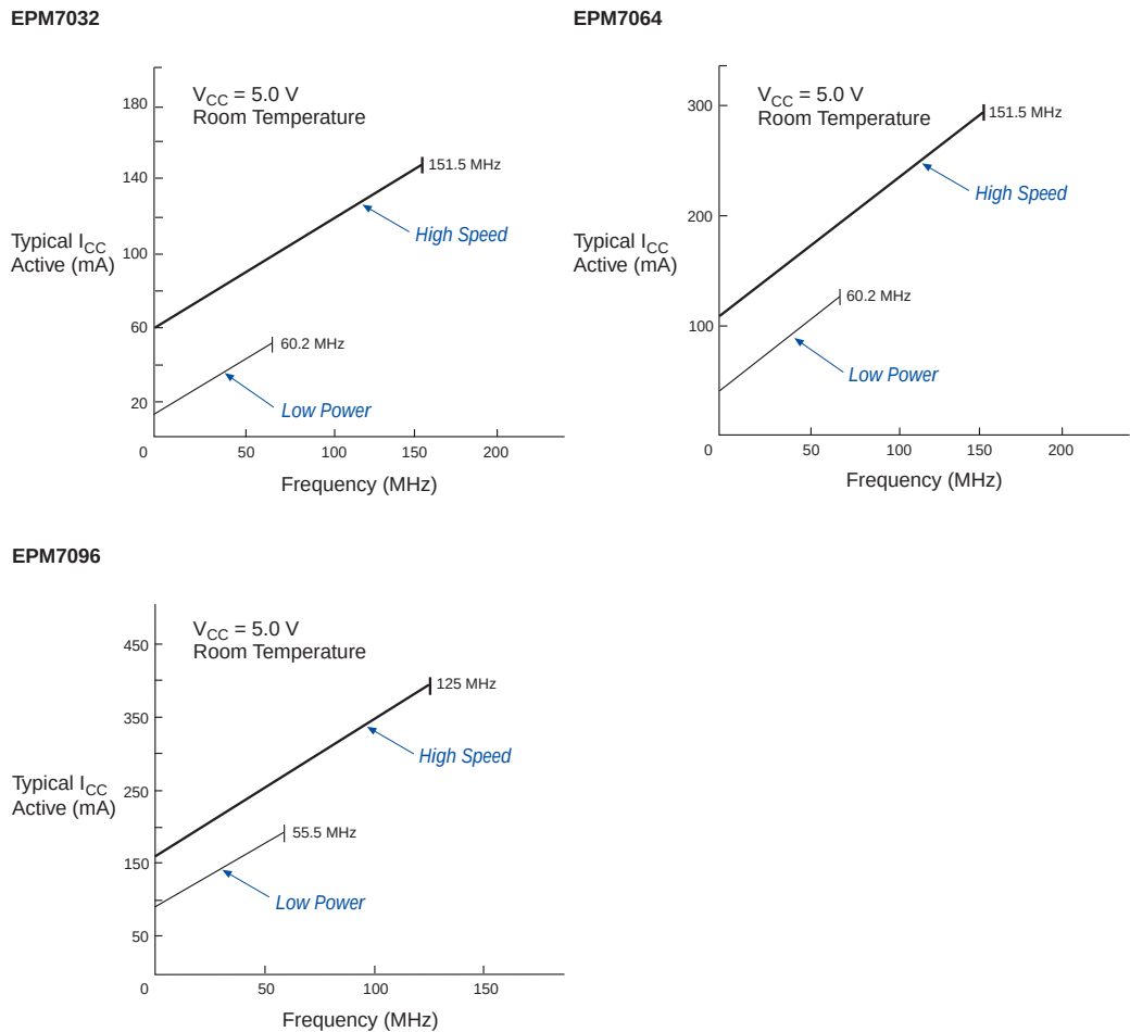
Figure 14. I_{CC} vs. Frequency for MAX 7000 Devices (Part 1 of 2)
