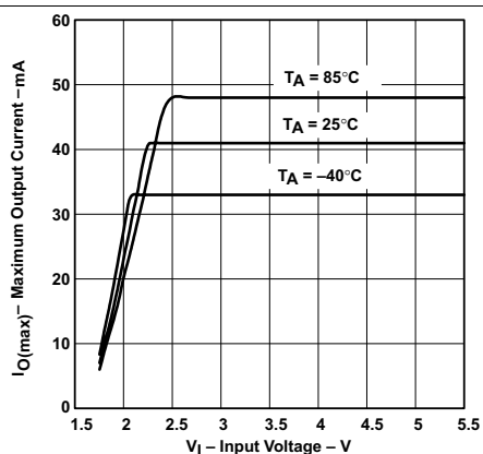
Figure 23. TPS60240 Maximum Output Current vs Input Voltage
