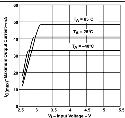
Figure 24. TPS60241 Maximum Output Current vs Input Voltage
