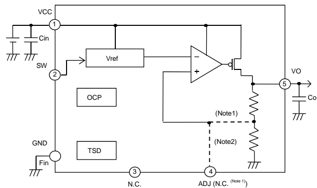
Figure 2. TO252-5
