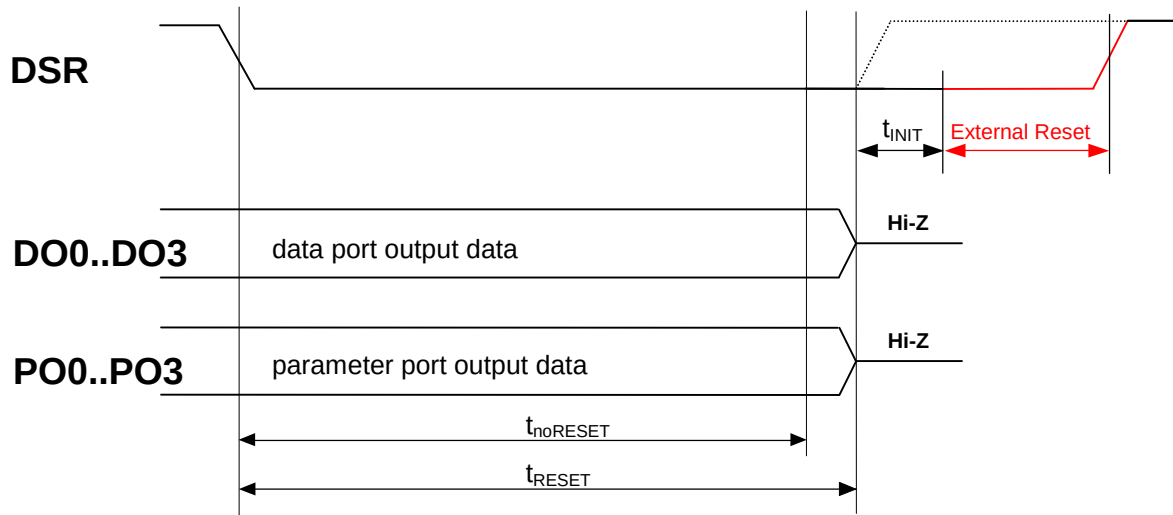
Figure 10: Timing diagram external Reset via \text{DSTBn}
