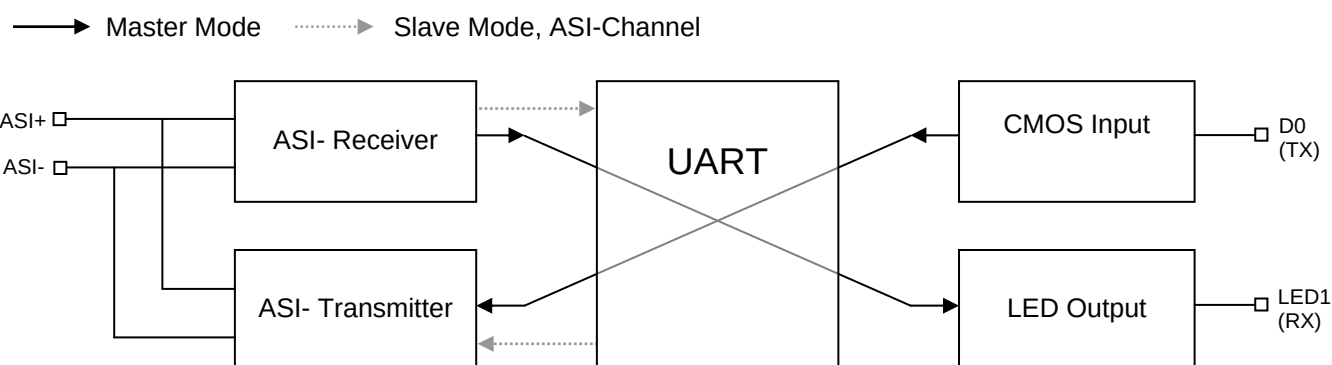
Figure 4: Data path in Master-, Repeater- and Monitor-Mode
