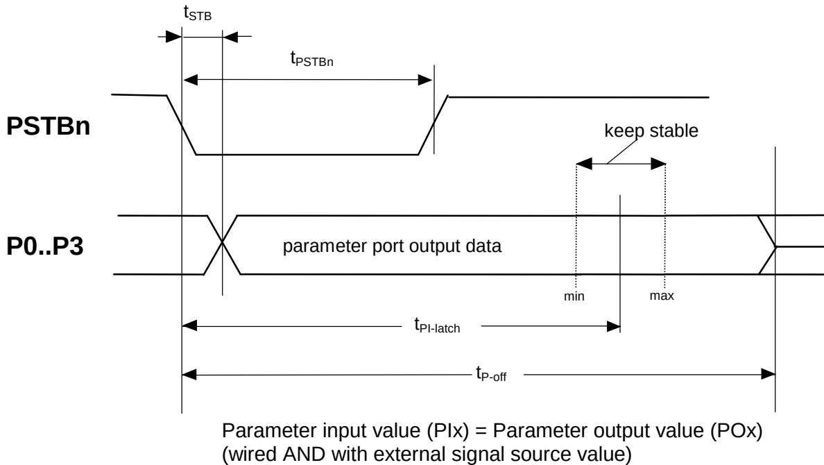
Figure 6: Timing Diagram Parameter Port P0 ... P3, PSTBn
