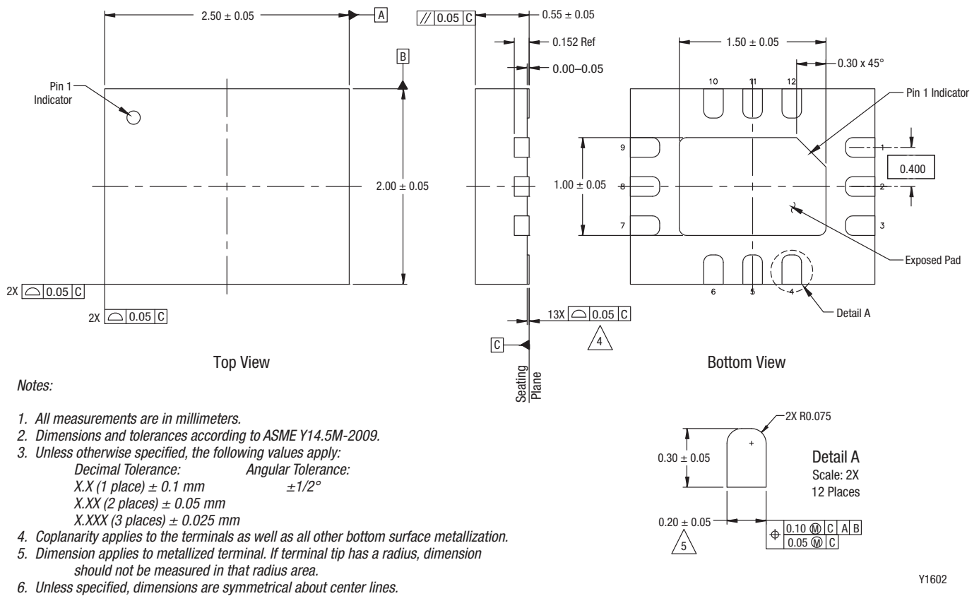
Figure 20. SE2433T Package Dimensions
